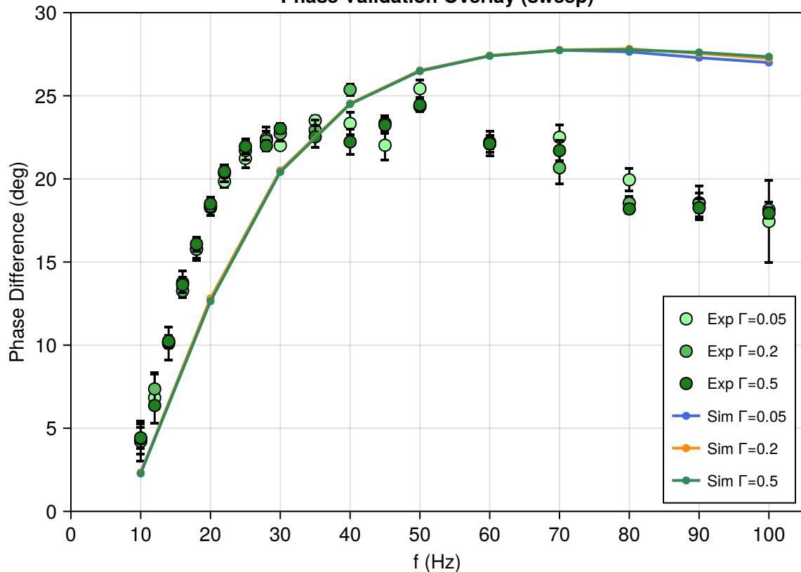
Phase Validation Overlay (sweep)
