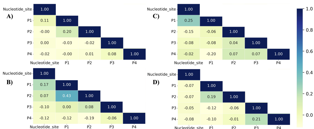
Figure S2: Pearson's Correlation for the volume fluctuations among different pockets and the effect of GEF binding. A) PREX1-bound Rac1; B) TIAM1-bound Rac1; C) VAV1-bound Rac1; D) DOCK2-bound Rac1. Rac1 in all GEF-bound systems is in the nucleotide-free state.
