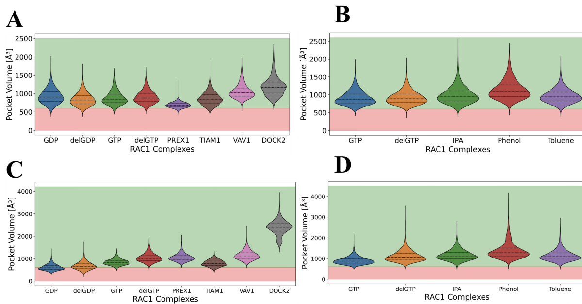
Figure S4: Analysis of pocket volume changes by combining pockets P1 with P2, and P3 with P4. A Combined pocket volume analysis for site P1+P2 ; B Combined pocket volume analysis for site P1+P2 in co-solvent; C Combined pocket volume analysis for site P3+P4; D Combined pocket volume analysis for site P3+P4 in co-solvent.
