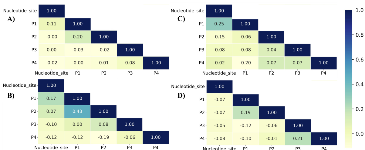
Figure S2: Pearson's Correlation for the volume fluctuations among different pockets and the effect of GEF binding. A PREX1-bound Rac1; B TIAM1-bound Rac1; C VAV1-bound Rac1; D DOCK2-bound Rac1. Rac1 in all GEF-bound systems is in the nucleotide-free state.
