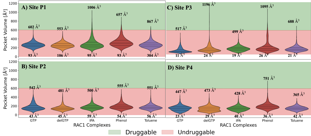
Figure 3: Accelerating transient pocket opening by cosolvent MD simulations.
