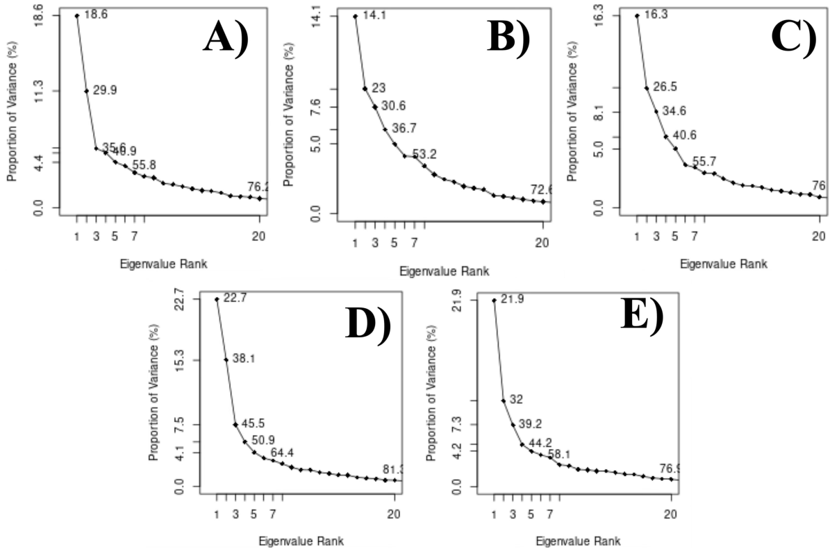
Figure S3: Scree plot to compute the cumulative variance explained by principal components. A) apo-Rac1 in TIP3P water box; B) GTP-bound Rac1 in TIP3P water box; C) apo-Rac1 in TIP3P water+isopropanol box; D) apo-Rac1 in TIP3P water+phenol box; E) apo-Rac1 in TIP3P water+toluene box.
