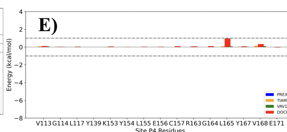
Figure 6: MMGBSA per residue decomposition analysis of residues on the Rac1 protein in complex with various GEFs. A) Per residue decomposition analysis for full Rac1 protein. The P-loop region is depicted in the magenta colour. The Switch I region is depicted in Orange Colour, and the Green coloured region is the Switch II region. The helical region is shown in yellow colour. The residue W56 is marked due to its biological importance in the GEF binding B) Per residue decomposition analysis for Site P1 residues. C) Per residue decomposition analysis for Site P2 residues. D) Per residue decomposition analysis for Site P3 residues. E) Per residue decomposition analysis for Site P4 residues. The "dot-dash" line indicates an arbitrary cutoff placed at \pm 1 kcal/mol, which suggests that energy values outside this region contribute significantly to the binding of GEFs.
