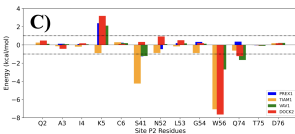
Figure 6: MMGBSA per residue decomposition analysis of residues on the Rac1 protein in complex with various GEFs. A) Per residue decomposition analysis for full Rac1 protein. The P-loop region is depicted in the magenta colour. The Switch I region is depicted in Orange Colour, and the Green coloured region is the Switch II region. The helical region is shown in yellow colour. The residue W56 is marked due to its biological importance in the GEF binding B) Per residue decomposition analysis for Site P1 residues. C) Per residue decomposition analysis for Site P2 residues. D) Per residue decomposition analysis for Site P3 residues. E) Per residue decomposition analysis for Site P4 residues. The "dot-dash" line indicates an arbitrary cutoff placed at \pm 1 kcal/mol, which suggests that energy values outside this region contribute significantly to the binding of GEFs.
