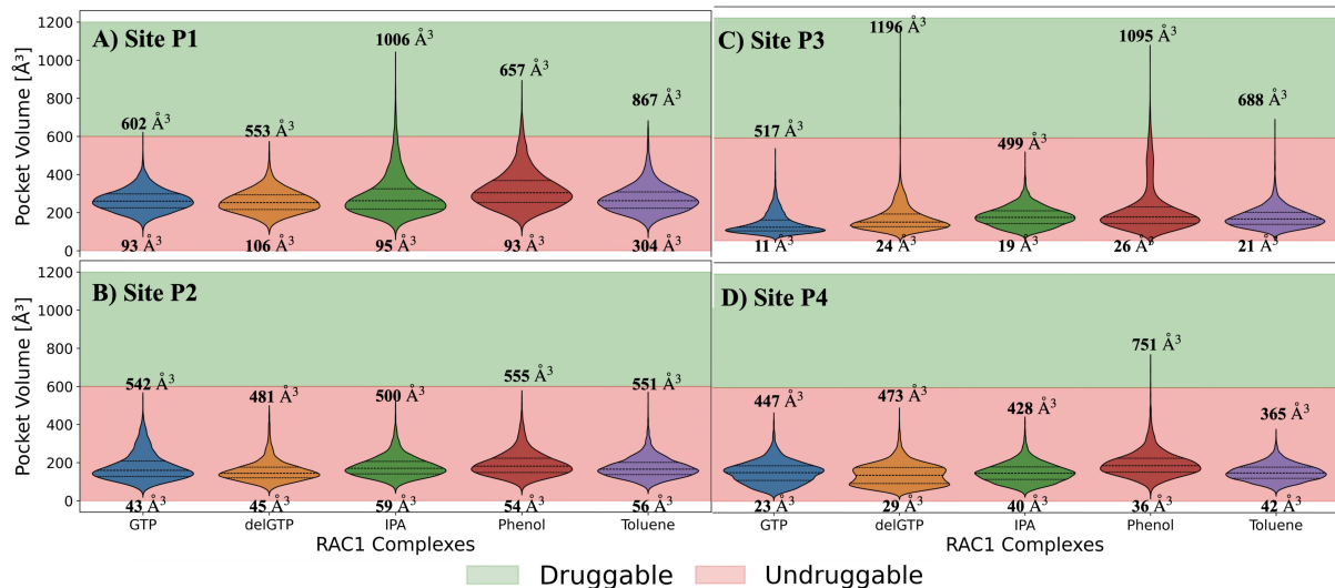
Figure 4: Accelerating transient pocket opening by cosolvent MD simulations.
