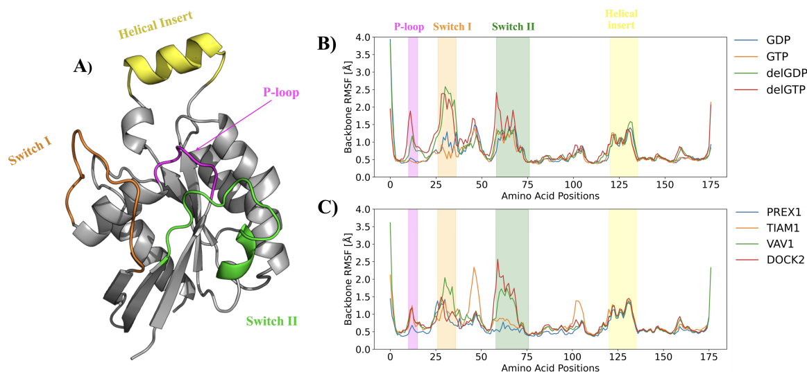
Figure 2: Rac1 domains and dynamics of each region. A) A Cartoon representation of human Rac1 (PDB id:1HE1). The P-loop region is depicted in the magenta colour. The Switch I region is depicted in Orange Colour, and the Green coloured region is the Switch II region. The helical region is shown in yellow colour. B) Atomic fluctuations of the backbone atoms are measured as root-mean-squared fluctuations (RMSF) for the human Rac1 domain to compare the effect of nucleotide binding on the dynamics of various domains. delGDP and delGTP are systems created by deleting the nucleotides from the Rac1 binding pocket to create corresponding apo system. C) Atomic fluctuations of the backbone atoms are measured as root-mean-squared fluctuations (RMSF) for the human Rac1 domain to compare the effect of GEF binding on the dynamics of various domains.
