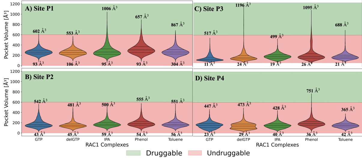
Figure 4: Accelerating transient pocket opening by cosolvent MD simulations.
