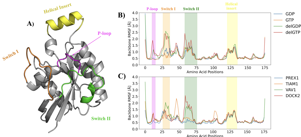
Figure 4: Rac1 domains and dynamics of each region. A) A Cartoon representation of human Rac1 ( PDB id:1HE1 ). The P-loop region is depicted in the magenta colour. The Switch I region is depicted in Orange Colour, and the Green coloured region is the Switch II region. The helical region is shown in yellow colour. B) Atomic fluctuations of the backbone atoms are measured as root-mean-squared fluctuations (RMSF) for the human Rac1 domain to compare the effect of nucleotide binding on the dynamics of various domains. delGDP and delGTP are systems created by deleting the nucleotides from the Rac1 binding pocket to create corresponding apo system. C) Atomic fluctuations of the backbone atoms are measured as root-mean-squared fluctuations (RMSF) for the human Rac1 domain to compare the effect of GEF binding on the dynamics of various domains.
