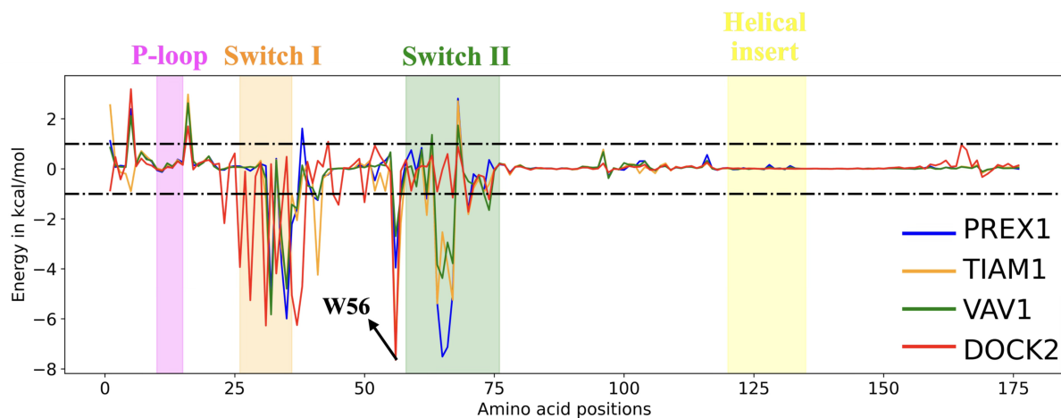
Figure 6: MMGBSA per residue decomposition analysis of residues on the RAC1 protein in complex with various GEFs. The P-loop region is depicted in the magenta colour. The Switch I region is depicted in Orange Colour, and the Green coloured region is the Switch II region. The helical region is shown in yellow colour
