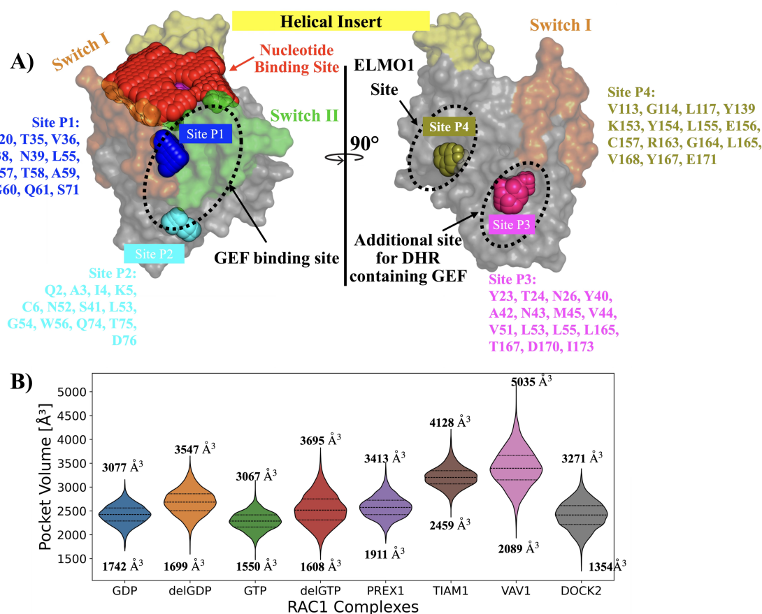
Figure 1: A) Rac1 surface with all possible binding pockets. The yellow-coloured region depicts the helical insert, which is peculiar to the Rho GTPase family. The orange-colored region depicts switch I, and the green colored region is switch II. Red spheres occupy the nucleotide-binding site. The pink-colored region is the P-loop. Blue spheres depict Site P1, cyan spheres show Site P2. Magenta spheres occupy the Site P3, and asparagus spheres show the Site P4. B) The violin plot illustrates the distribution of the pocket volumes for each of the nucleotide-binding sites. The changes in the pocket volumes are monitored when Rac1 is complexed with either GEFs, GDP, GTP or in the apo -states named as delGDP (GDP deleted from GDP-bound system), and delGTP (GDP deleted from GTP-bound system). The amino acid numbering for Rac1 follows the uniprot id: P63000.
