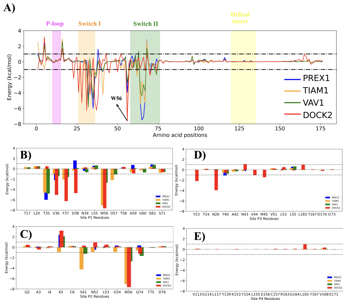
Figure 6: MMGBSA per residue decomposition analysis of residues on the RAC1 protein in complex with various GEFs. The P-loop region is depicted in the magenta colour. The Switch I region is depicted in Orange Colour, and the Green coloured region is the Switch II region. The helical region is shown in yellow colour
