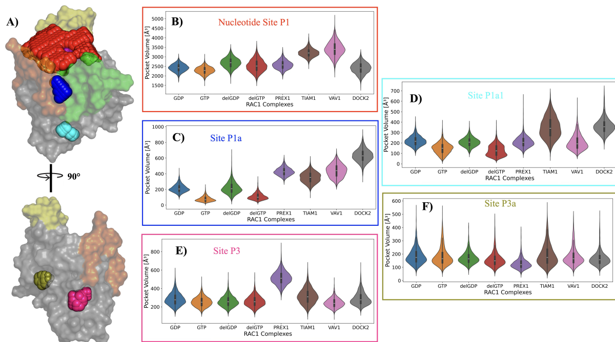
Figure 1: Binding Pockets on RAC1 surface. A) B) C) D) E) F) F)
