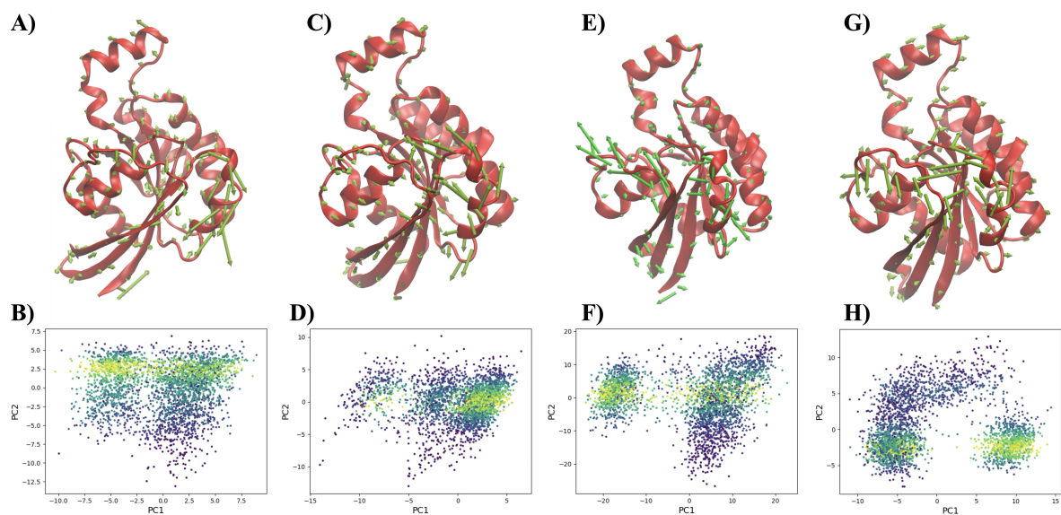
Figure 4: Essential Dynamics of RAC1 protein extracted using principal component analysis.
