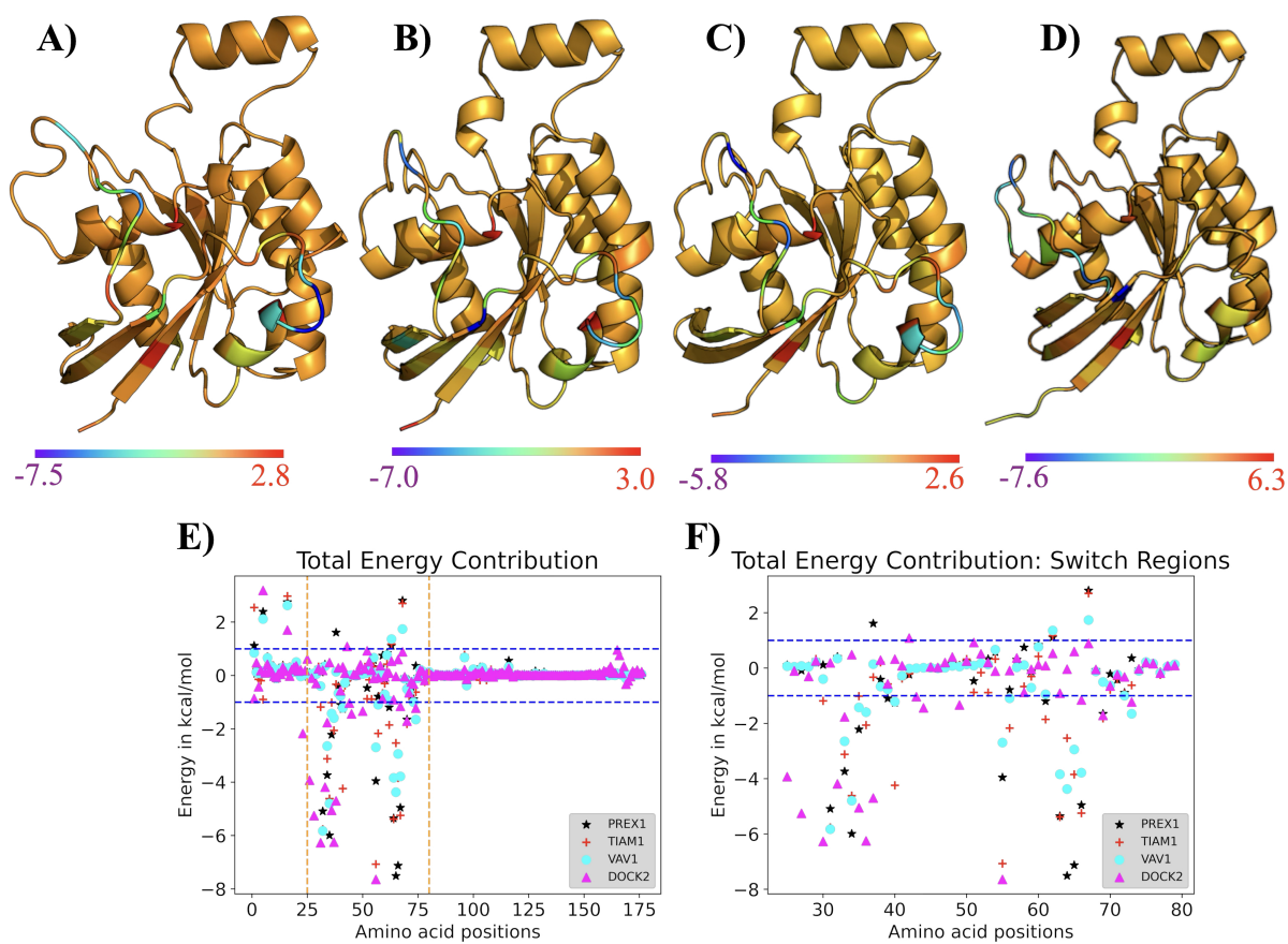
Figure 6: Per Residue contribution from RAC1 protein towards GEF binding.
