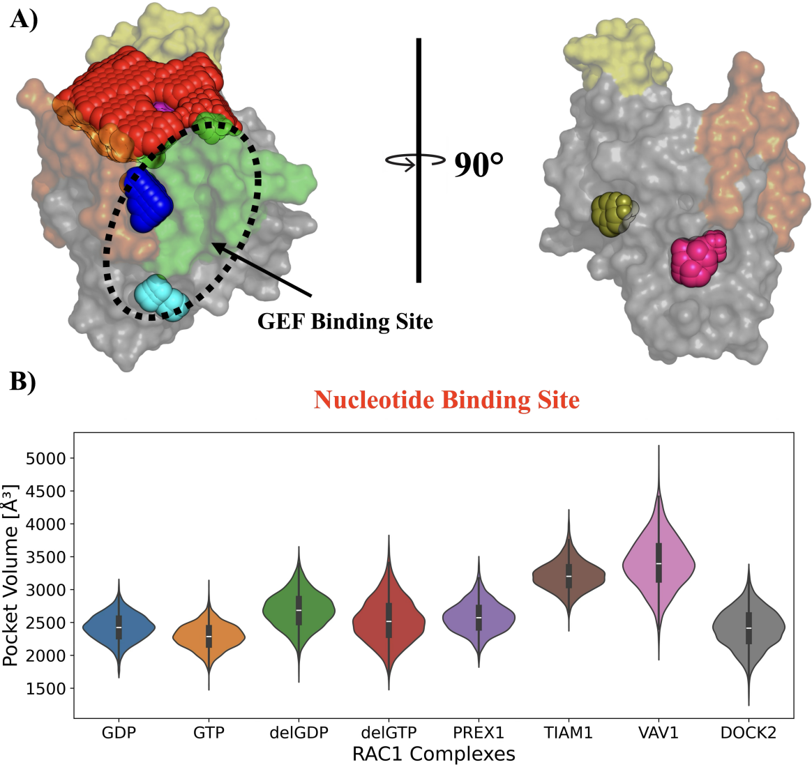
Figure 1: Binding Pockets on RAC1 surface. A) Shows the surface model of Rac1 protein with coloured spears illustrating the binding site identified with POVME2. The helical insert is highlighted using the yellow colour. The green region indicates the switch II and orange region indicates the switch I region. The magenta region slightly visible through the red spears indicates the P-loop. The red spears occupy the nucleotide binding site that is lined with helical insert, switch regions and the P-loop forms the phosphate binding region. Blue spears occupy the site P1a and the cyan spears occupy the site P1a1. Site P3 and P3a are visible by rotating the Rac1 by 90°. The salmon pink spears occupy site P3 while the olive green spears occupy site P3a. The violin plots illustrate the distribution of the pocket volumes for each of the binding sites on the Rac1 surface. The changes in the pocket volumes are monitored when Rac1 is complexed with either GEFs, GDP, GTP or in the apo -state. B) Site P1 or the nucleotide binding site C) Site P1a D) Site P1a1 E) Site P3 and F) Site P3a
