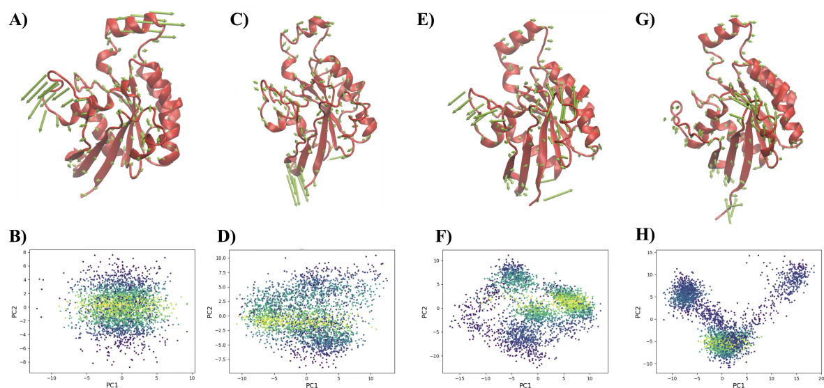
Figure 5: Essential Dynamics of RAC1 protein extracted using principal component analysis.
