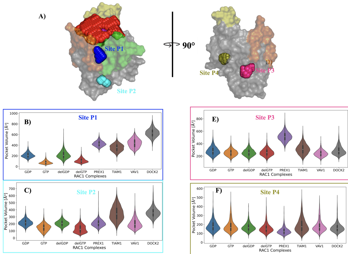
Figure 2: Binding Pockets on RAC1 surface. A) Shows the surface model of Rac1 protein with coloured spears illustrating the binding site identified with POVME2. The helical insert is highlighted using the yellow colour. The green region indicates the switch II and orange region indicates the switch I region. The magenta region slightly visible through the red spears indicates the P-loop. The red spears occupy the nucleotide binding site that is lined with helical insert, switch regions and the P-loop forms the phosphate binding region. Blue spears occupy the site P1a and the cyan spears occupy the site P1a1. Site P3 and P3a are visible by rotating the Rac1 by 90°. The salmon pink spears occupy site P3 while the olive green spears occupy site P3a. The violin plots illustrate the distribution of the pocket volumes for each of the binding sites on the Rac1 surface. The changes in the pocket volumes are monitored when Rac1 is complexed with either GEFs, GDP, GTP or in the apo -state. B) Site P1 or the nucleotide binding site C) Site P1a D) Site P1a1 E) Site P3 and F) Site P3a
