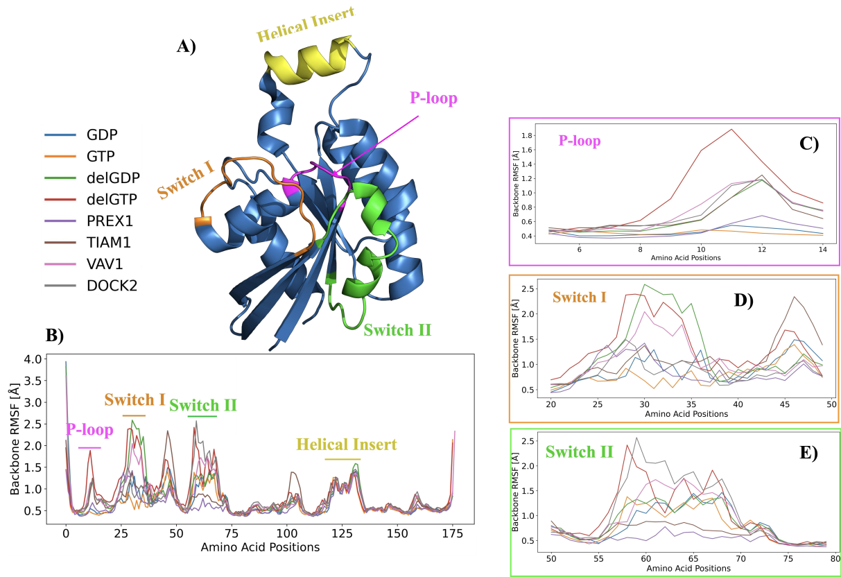
Figure 3: RAC1 domains and dynamics of each region. A) A Cartoon representation of human RAC1 (PDB id:1HE1). The P-loop region is depicted in the magenta colour. The Switch I region is depicted in Orange Colour, and the Green coloured region is the Switch II region. The helical region is shown in yellow colour. B) Atomic fluctuations of the backbone atoms are measured as root-mean-squared fluctuations (RMSF) for human RAC1 domain. C) Backbone atom RMSF is shown as the expansion of the P-loop region. D) Backbone atom RMSF is shown as the expansion of the Switch I region. E) Backbone atom RMSF is shown as the expansion of the Switch II region. F) The normalised distribution of the root-mean-squared deviation of the backbone atoms of the P-loop. G) The normalised distribution of the root-mean-squared deviation of the backbone atoms of the Switch I region. H) The normalised distribution of the root-mean-squared deviation of the backbone atoms of the Switch II region. delGDP and delGTP are systems from which by deleting the corresponding nucleotides from the RAC1 binding pocket to create an apo system.
