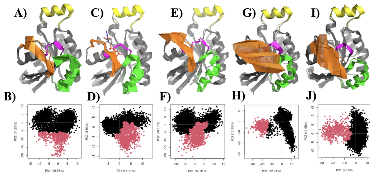
Figure 5: Essential Dynamics of Rac1 protein to explain the opening and closing of the transient pockets induced by the cosolvent probes. A) apo -Rac1 in TIP3P water box. B) Identification of apo -Rac1 conformational clusters in TIP3P water box based on essential dynamics using first two PCs. C) GTP-bound Rac1 in TIP3P water box. D) Identification of GTP-bound Rac1 conformational clusters in TIP3P water box based on essential dynamics using first two PCs. E) apo -Rac1 in TIP3P water+Isopropanol box. F) Identification of apo -Rac1 conformational clusters in water+Isopropanol box based on essential dynamics using first two PCs. G) apo -Rac1 in TIP3P water+Phenol box. H) Identification of apo -Rac1 conformational clusters in TIP3P water+Phenol box based on essential dynamics using first two PCs. I) apo -Rac1 in TIP3P water+Toluene box. J) Identification of apo -Rac1 conformational clusters in TIP3P water+Toluene box based on essential dynamics using first two PCs. Magenta colour indicates the P-loop region. Orange colour indicates switch I region. Green colour indicates switch II region. Yellow colour indicates helical insert.
