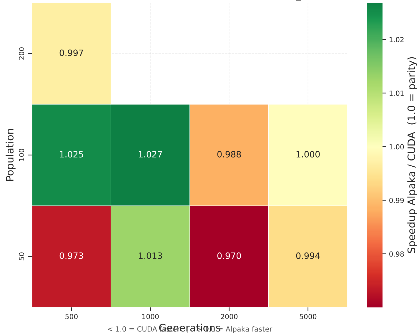
Relative Speedup: Alpaka vs CUDA — small_multi
