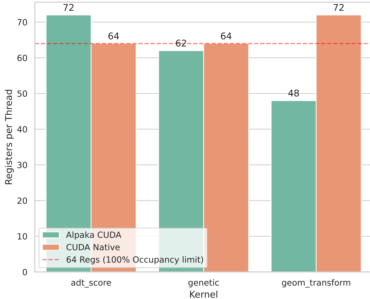
Register Usage per Kernel (Lower is Better)
