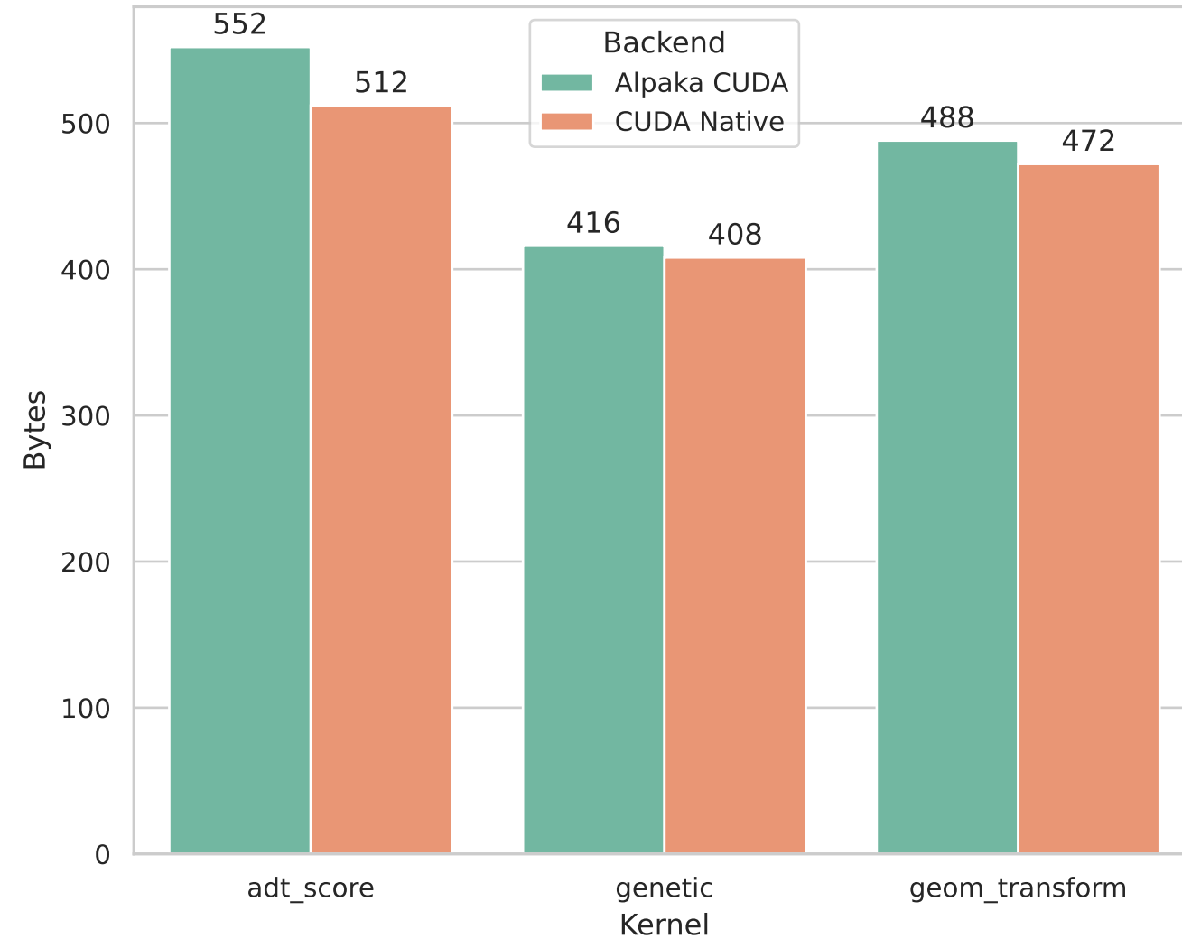
Constant Memory Usage (Bytes)
