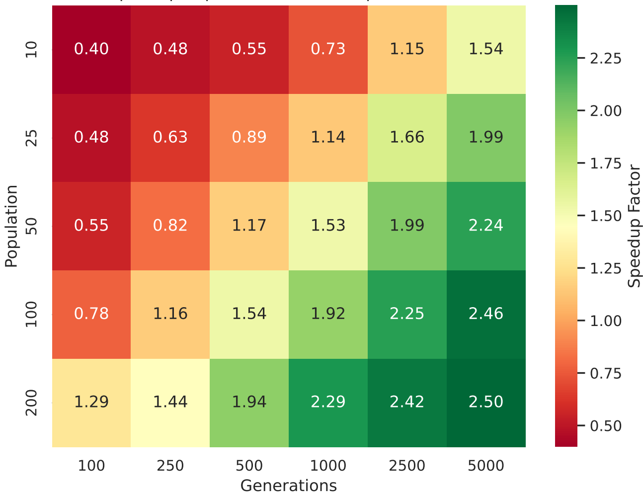
The Cost of Unrolling on CPU Speedup: Alpaka (No-Unroll) / Alpaka (Unroll)
