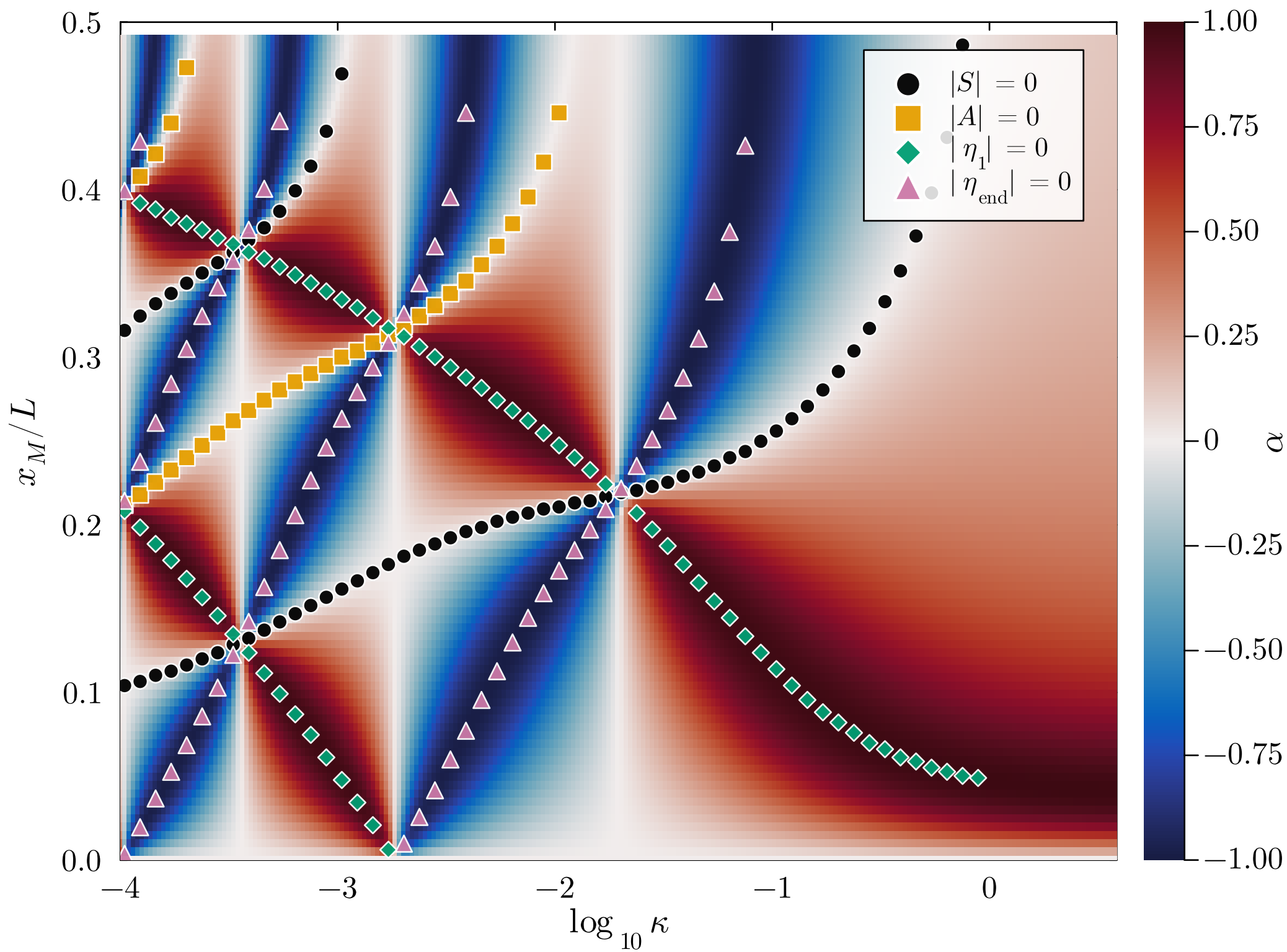
Coupled raft, \Lambda = 0.60 — a-priori prediction
