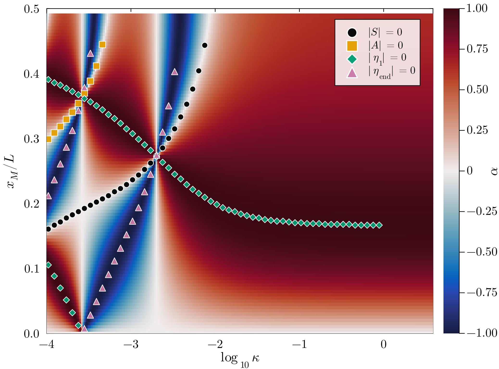
Uncoupled raft, \Lambda = 0 — a-priori prediction
