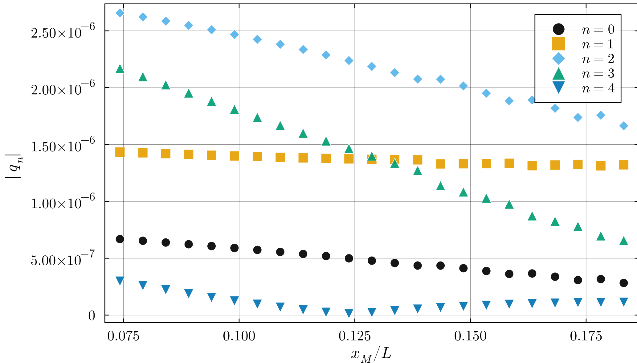
Modal amplitudes on |\eta_{\text{end}}| = 0 curve (\alpha < -0.99, \text{ coupled; } \log_{10} \kappa > -2.8, x_M/L < 0.25)
