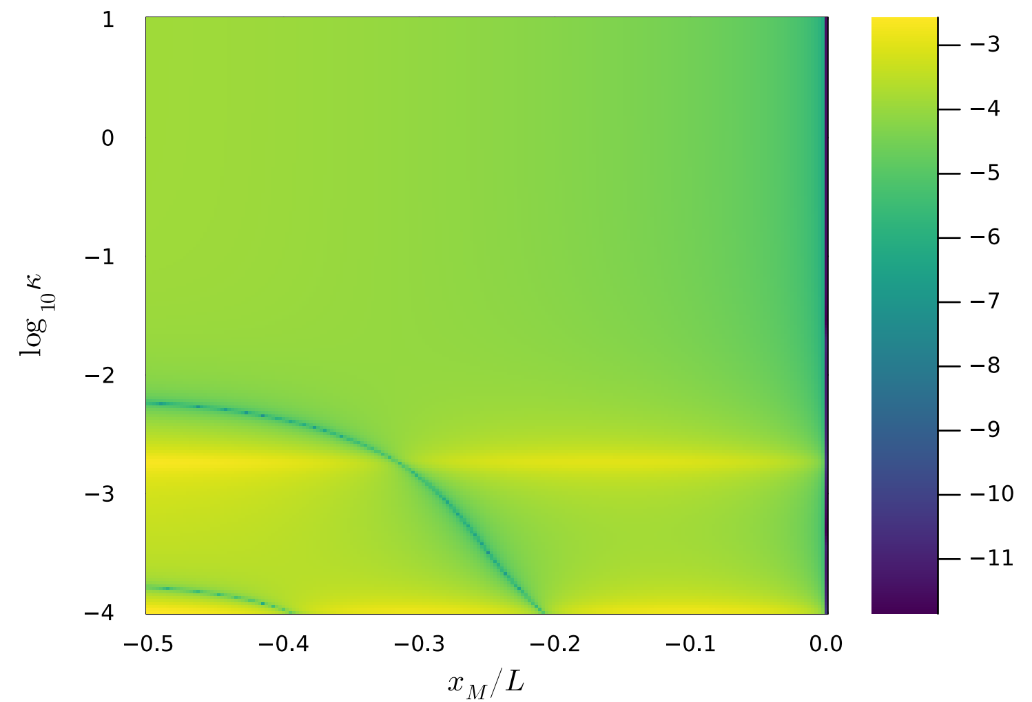
\log_{10}|A|
