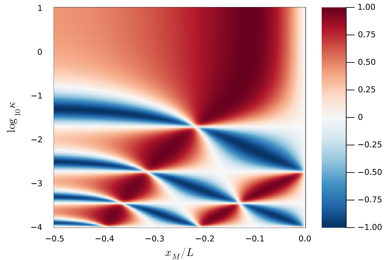
\alpha (for reference)
