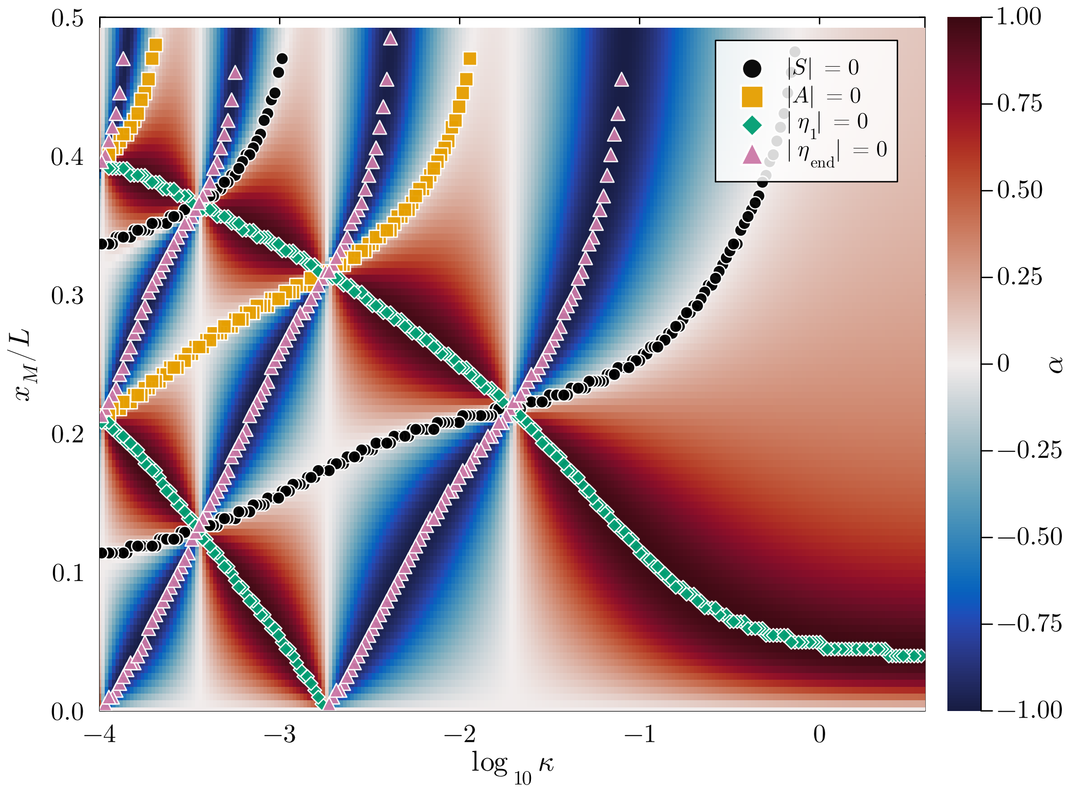
Coupled raft, \Lambda = 0.60 — direct integration
