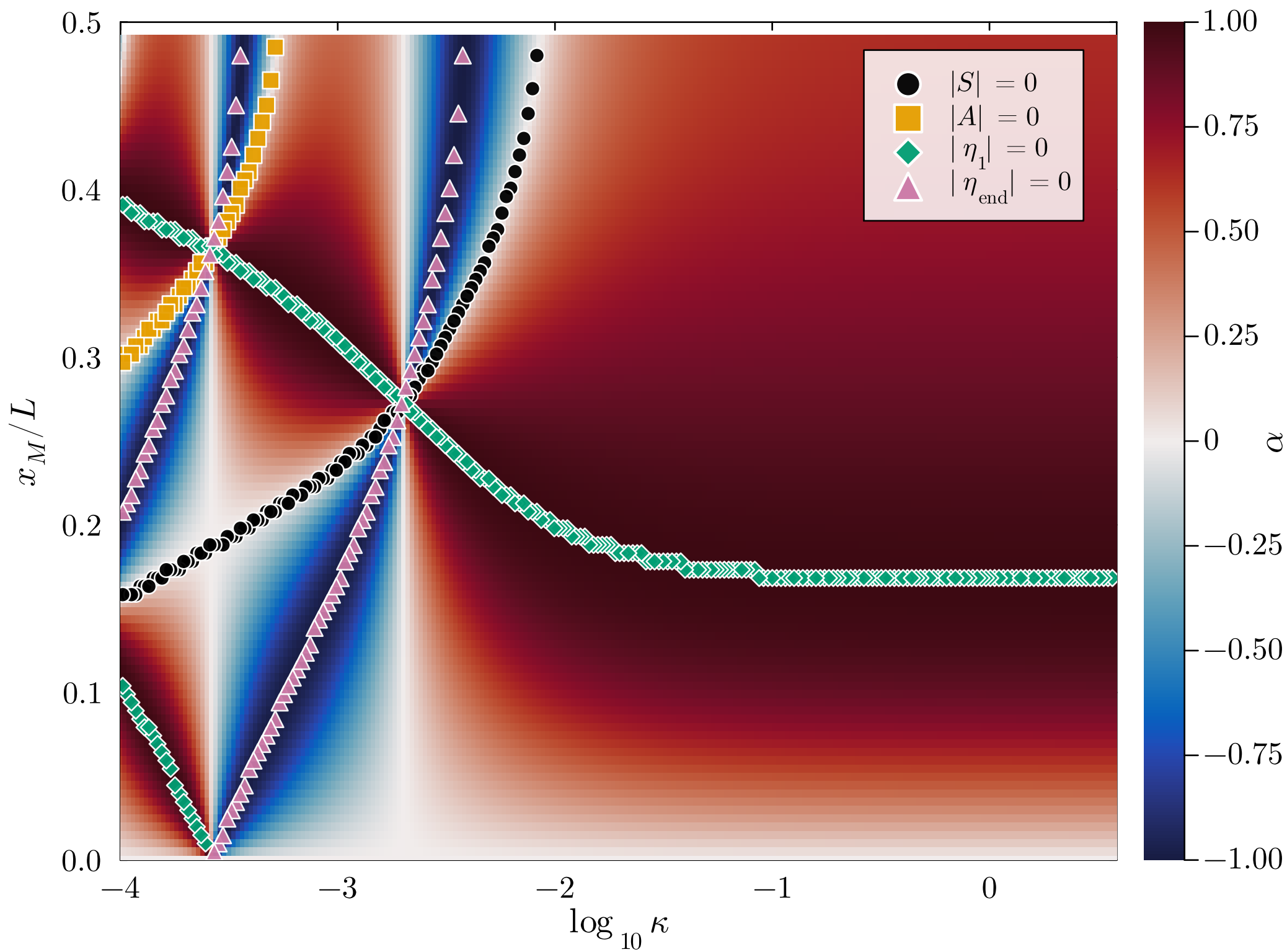
Uncoupled raft, \Lambda = 0 — direct integration
