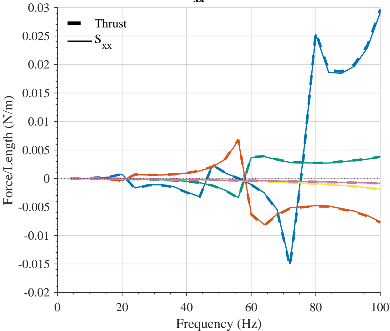
Thrust vs. S_{xx} (Radiation Stress)
