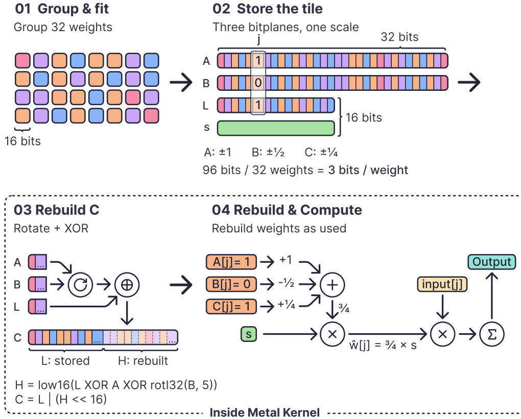
Figure 1: MORPH32-c, the coupled layout. Each tile stores two full sign planes, half of a third, and one scale. The Metal kernel reconstructs the missing bits with rotation and XOR before using the weights. A compact tile takes 96 bits; the deployed profile mixes compact and full tiles.
