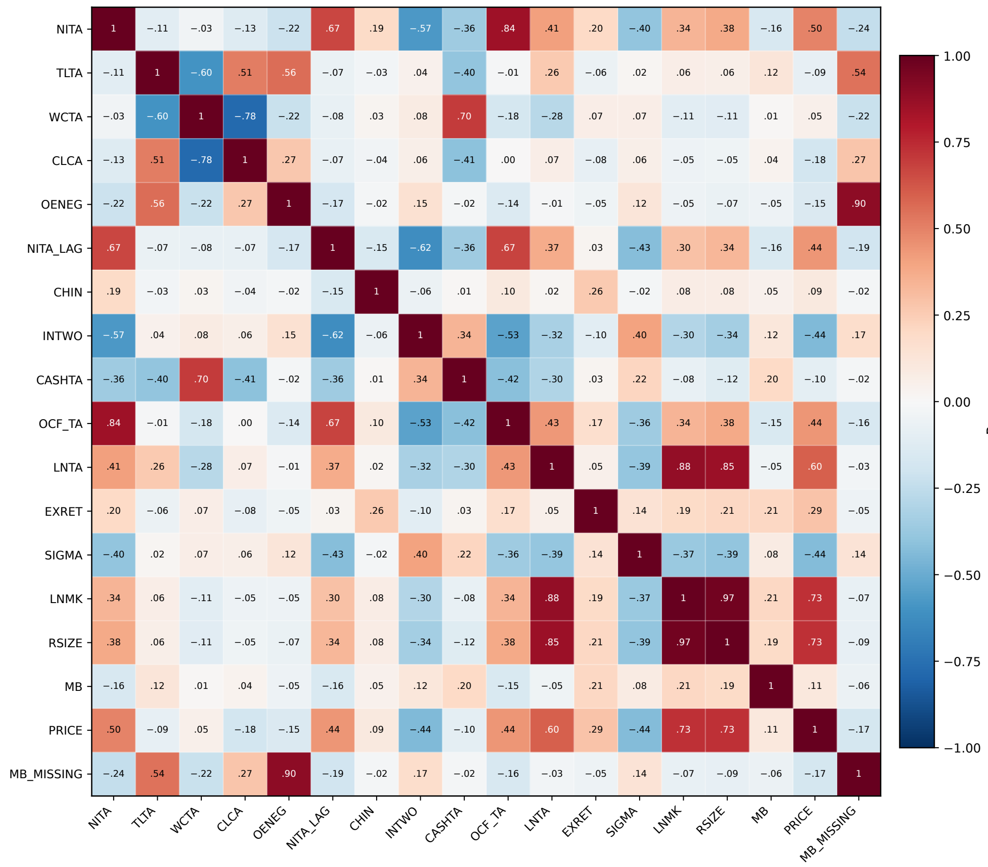
Pairwise Pearson Correlation Matrix
