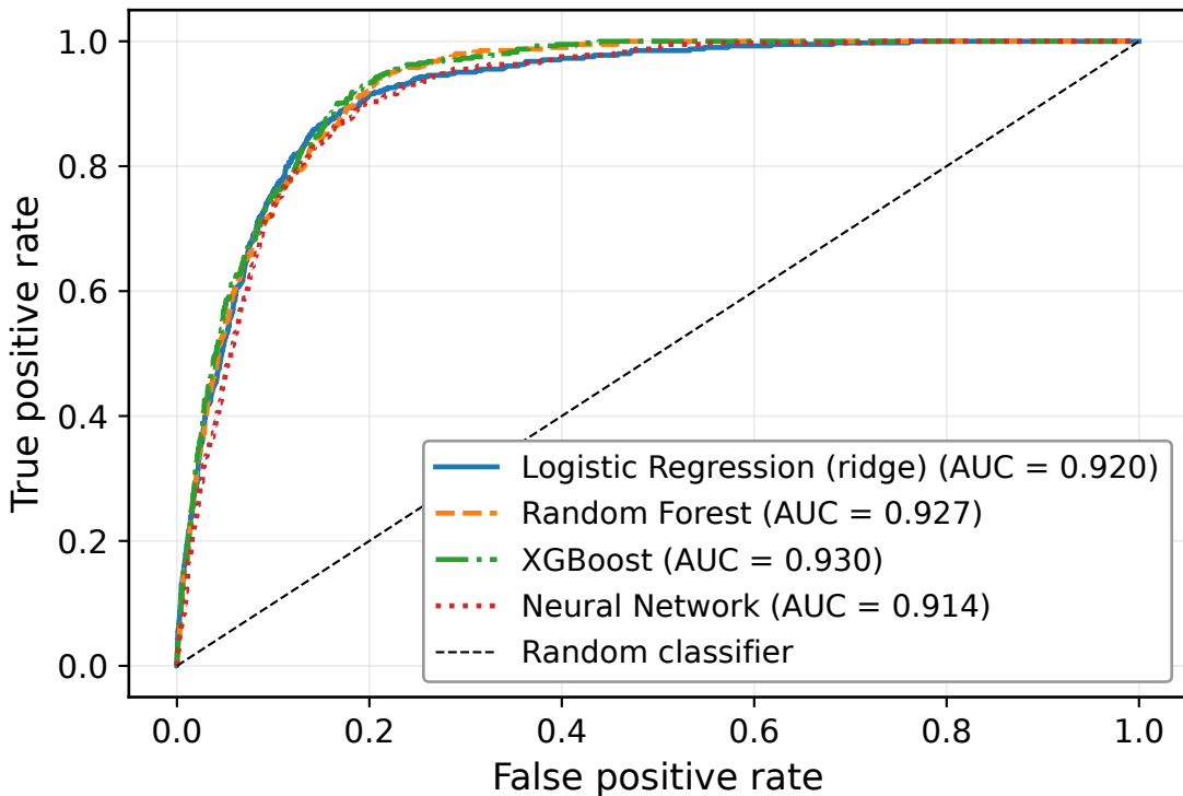
ROC Curves (Test Sample)
