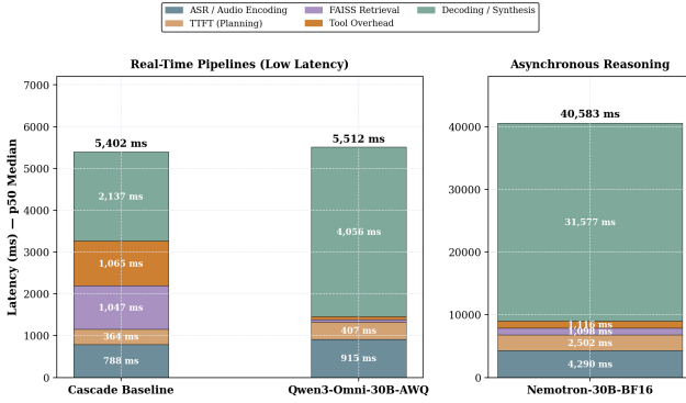
Figure 3: Latency breakdown by generation stage ( p_{50} medians) showing the operational speed of Cascade Baseline compared to the reasoning-intensive cycles of Nemotron-3-Nano-Omni.
