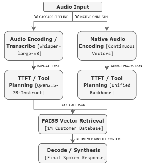
Figure 1: Architectural execution pathways of the modular Cascade baseline (A) versus the unified, native Omni-SLM pipeline (B) integrated with an intermediate FAISS customer database retrieval loop.
