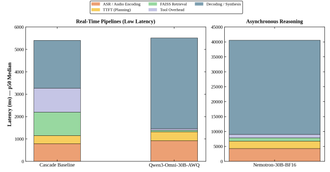
Figure 3: Latency breakdown by generation stage ( p_{50} medians) showing the operational speed of Cascade Baseline compared to the reasoning-intensive cycles of Nemotron-3-Nano-Omni.
