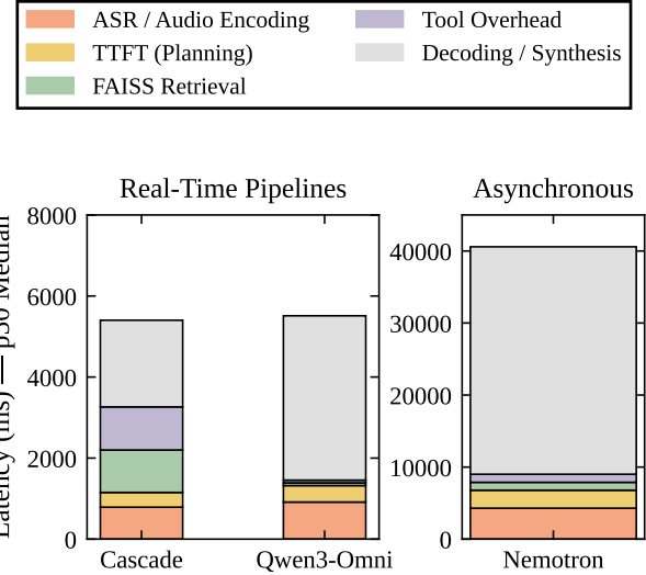
Figure 3: Latency breakdown by generation stage ( p_{50} medians) showing the operational speed of Cascade Baseline compared to the reasoning-intensive cycles of Nemotron-3-Nano-Omni.
