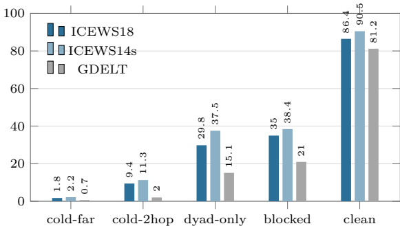
MRR ( \times 100 )
