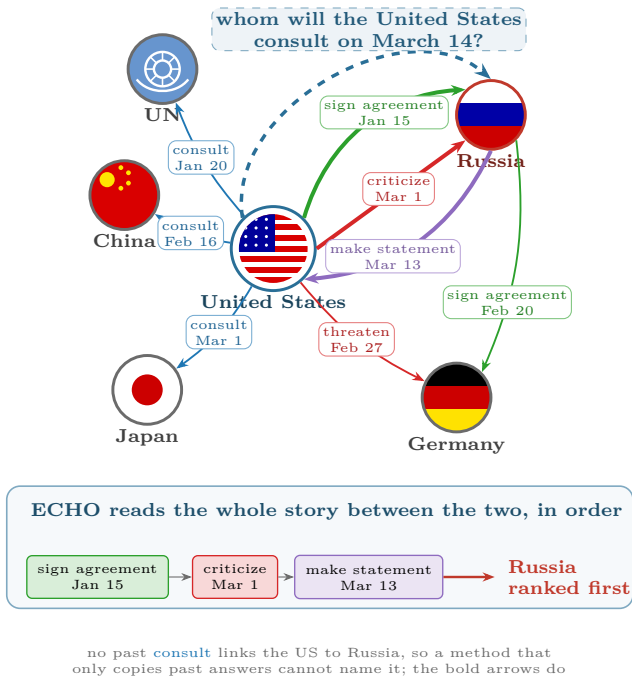
Figure 1: What ECHO reads. Countries linked by dated, typed events, and the question: whom will the United States consult on March 14? A copy mechanism reads only the thin consult arrows, so Russia is not a candidate for it. ECHO reads every event between the United States and each country as one ordered stream; for Russia that stream, an agreement, a criticism and a statement within weeks, says the two are in close contact, and ECHO ranks Russia first. On ICEWS18 the answer is visible only in this reading for 23.4% of test queries (Section 4). Names and dates are illustrative.
