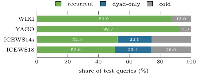
Figure 2: Strata are a property of the data. Share of test queries whose answer is recurrent (occurred with (s, r) before), dyad-only (never with (s, r) , but s and the answer interacted under another relation or direction) and cold (never interacted). A copy mechanism is silent on the dyad-only stratum by construction. It is a quarter of the ICEWS queries and absent from YAGO and WIKI.
