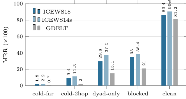
Figure 5: MRR by stratum on the three event datasets (three seeds). The profile is the same on all three: the clean stratum is solved, the blocked and dyad-only strata are where a copy mechanism fails and where ECHO earns its margin, and the two cold strata are where the remaining headroom lies. GDELT, whose fifteen-minute snapshots make every stratum sparser, is lower everywhere but keeps the ordering.
