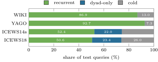
Figure 1: Strata are a property of the data. Share of test queries whose answer is recurrent (occurred with (s, r) before), dyad-only (never with (s, r) , but s and the answer interacted under another relation or direction) and cold (never interacted). A copy mechanism is silent on the dyad-only stratum by construction. It is a quarter of the ICEWS queries and absent from YAGO and WIKI.
