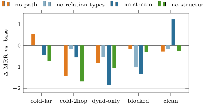
Figure 3: Where each part acts (ICEWS18, seed 1, change of MRR per stratum when the part is removed). The path intensity is paid for on cold-2hop; the relation types on blocked; the stream on dyad-only and blocked; the structural branch on both cold strata. Removing the whole dyadic branch costs 3.5 on dyad-only, 5.1 on blocked and 17.4 on clean, off the scale of this plot.
