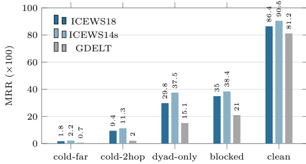
Figure 4: MRR by stratum on the three event datasets (three seeds). The profile is the same on all three: the clean stratum is solved, the blocked and dyad-only strata are where a copy mechanism fails and where ECHO earns its margin, and the two cold strata are where the remaining headroom lies. GDELT, whose fifteen-minute snapshots make every stratum sparser, is lower everywhere but keeps the ordering.
