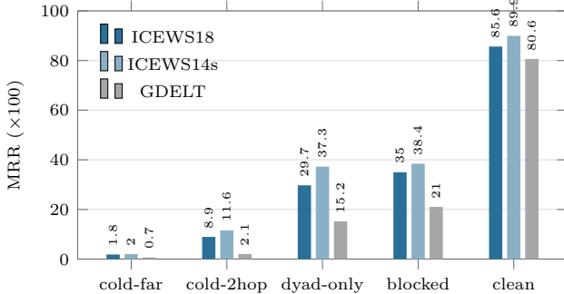
Figure 3: MRR by stratum on the three event datasets (three seeds). The profile is the same on all three: the clean stratum is solved, the blocked and dyad-only strata are where a copy mechanism fails and where ECHO earns its margin, and the two cold strata are where the remaining headroom lies. GDELT, whose fifteen-minute snapshots make every stratum sparser, is lower everywhere but keeps the ordering.
