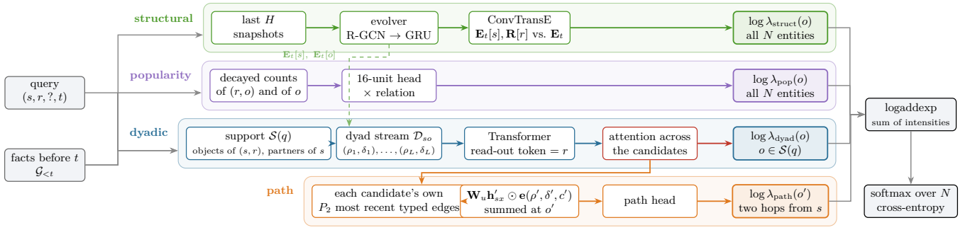
Figure 2: Overview of ECHO. A query (s, r, ?, t) is scored by four intensities that are added as intensities, never gated. The structural intensity evolves entity states through the last H snapshots and decodes against every entity. The popularity intensity scores every entity from multi-scale decayed counts of (r, o) and of o . The dyadic intensity builds the support of s , encodes each candidate’s typed event stream with a Transformer whose read-out token is the query relation, lets the candidates of the query attend to one another , and scores each one. The path intensity forwards every candidate’s state along that candidate’s own most recent typed edges and sums the messages arriving at each second-hop entity. The four log-intensities are combined by \text{logaddexp} and trained with one cross-entropy over all N entities.
