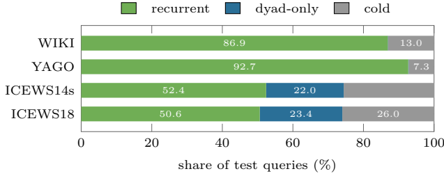
Figure 1: Strata are a property of the data. Share of test queries whose answer is recurrent (occurred with (s, r) before), dyad-only (never with (s, r) , but s and the answer interacted under another relation or direction) and cold (never interacted). A copy mechanism is silent on the dyad-only stratum by construction. It is a quarter of the ICEWS queries and absent from YAGO and WIKI.
