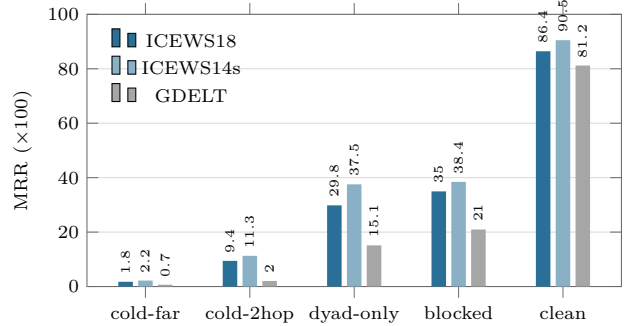
Figure 4: MRR by stratum on the three event datasets (three seeds). The profile is the same on all three: the clean stratum is solved, the blocked and dyad-only strata are where a copy mechanism fails and where ECHO earns its margin, and the two cold strata are where the remaining headroom lies. GDELT, whose fifteen-minute snapshots make every stratum sparser, is lower everywhere but keeps the ordering.
