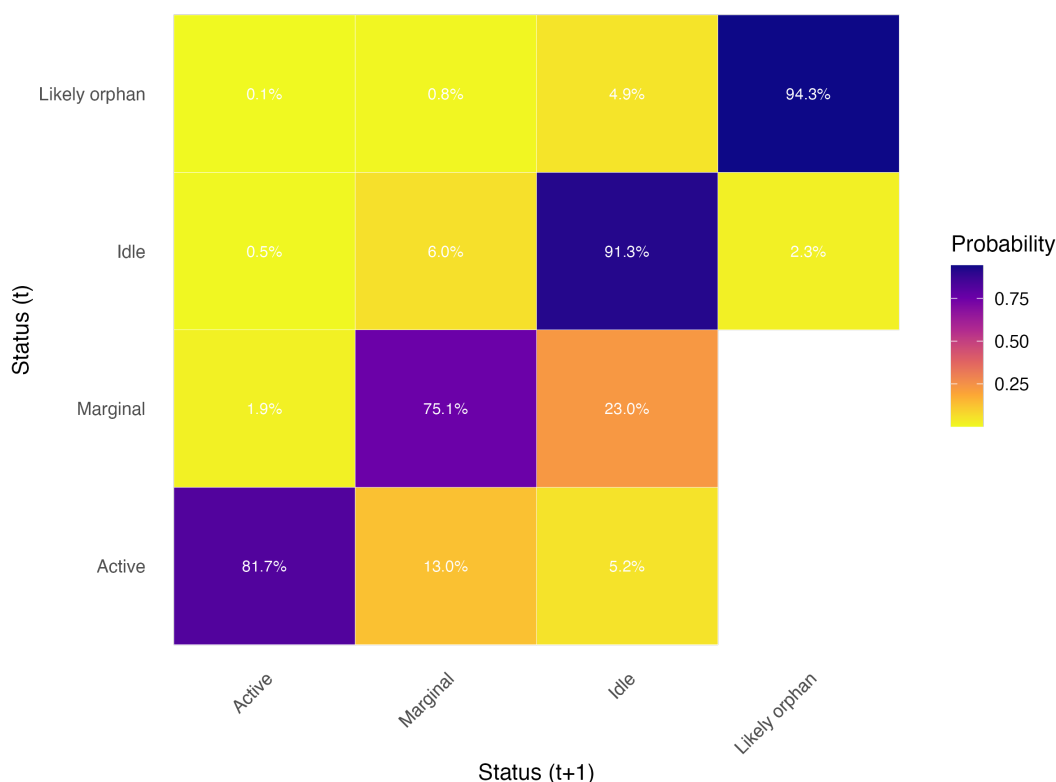
Figure 4.3: Transition Matrix
