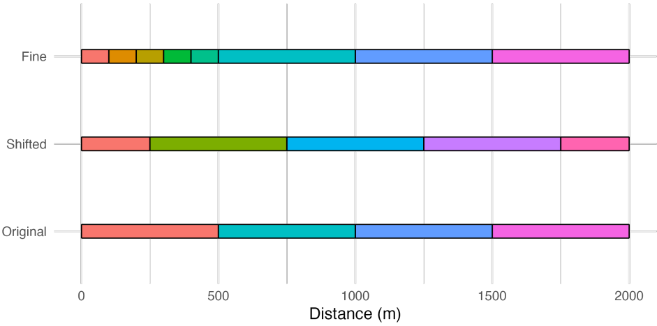
Figure 2.14: Comparison of Alternative Distance Bin Definitions
