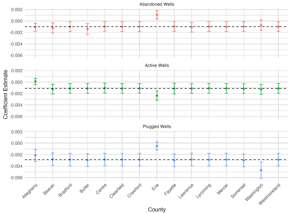
Figure 2.19: “Leave One County Out” Estimation
