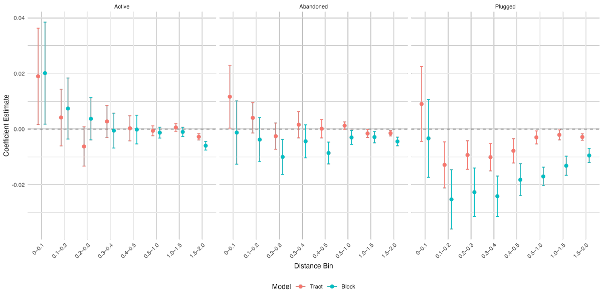
Figure 2.15: OLS Estimates with Finer Distance Bins
