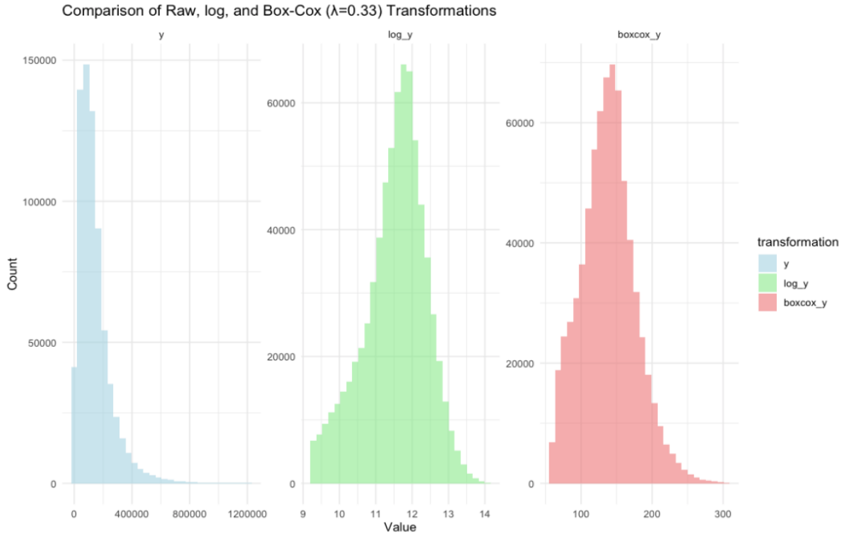
Figure 2.20: Distribution of Home Prices Under Log and Box-Cox Transformations
