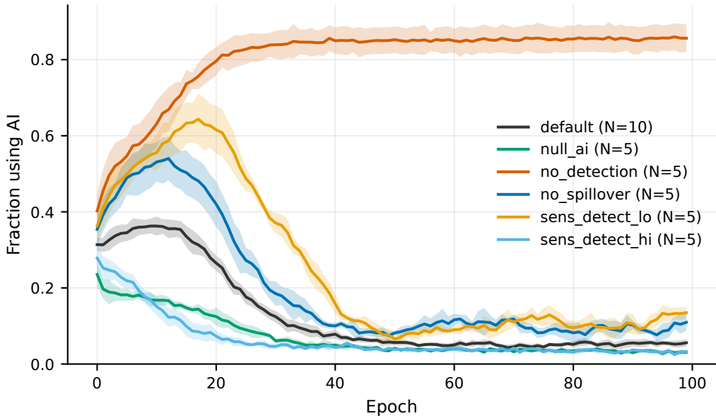
AI usage trajectory by arm (mean \pm 95% CI)
