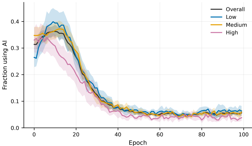
AI adoption over time (default, N=10 seeds, mean \pm 95% CI)
