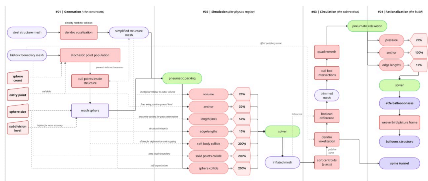
FIG 6.1 · The Grasshopper algorithm behind the inflation simulation, from constraints to Kangaroo goals to the settled cluster
