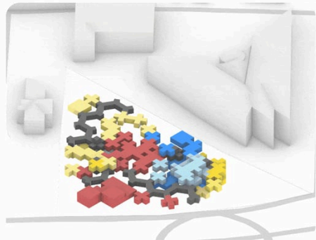
WASP | precise subprogram gradient
