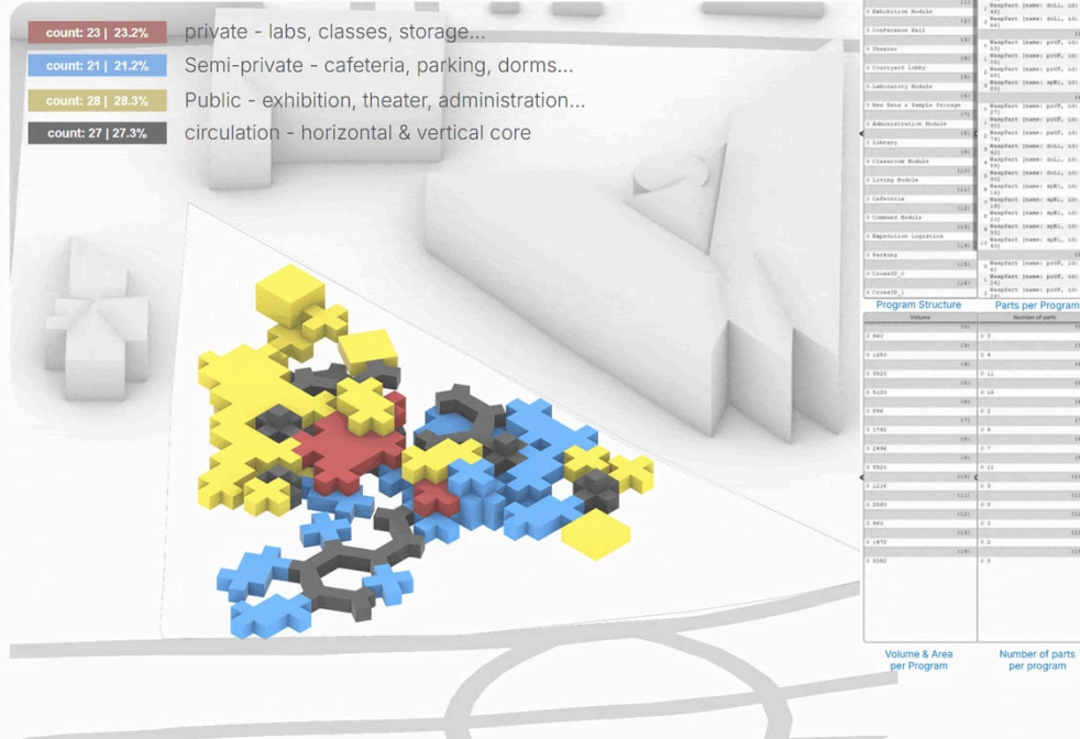
WASP | iterations
