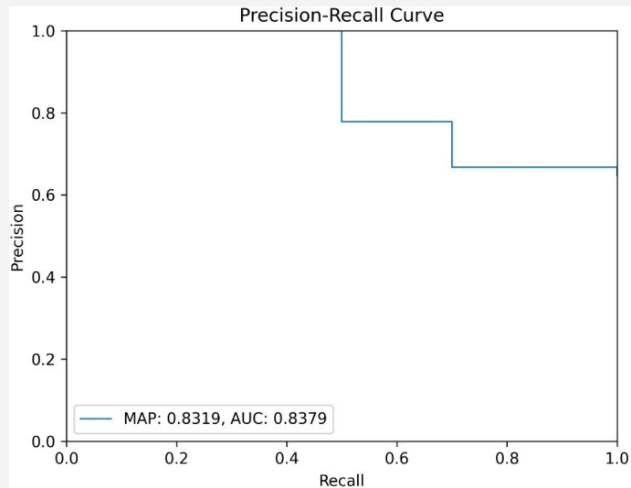
Query 3 - Improved Schema
