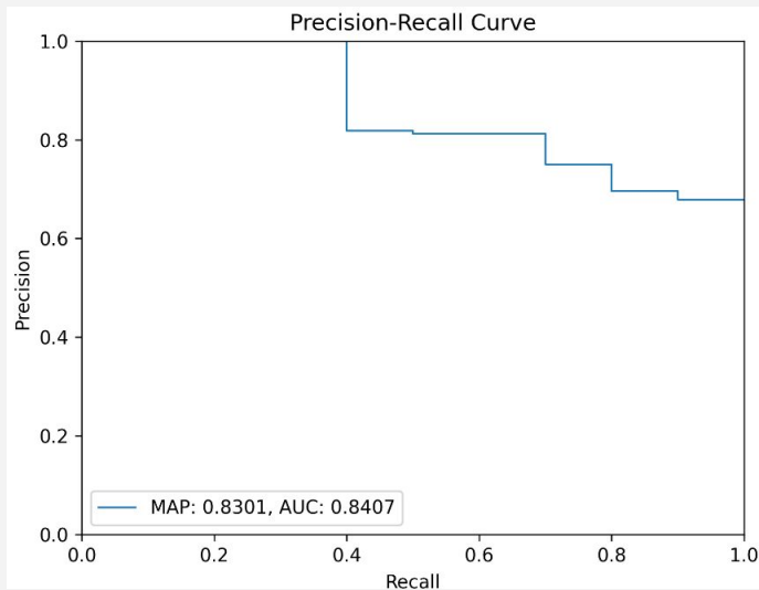
Query 4 - Improved Schema
