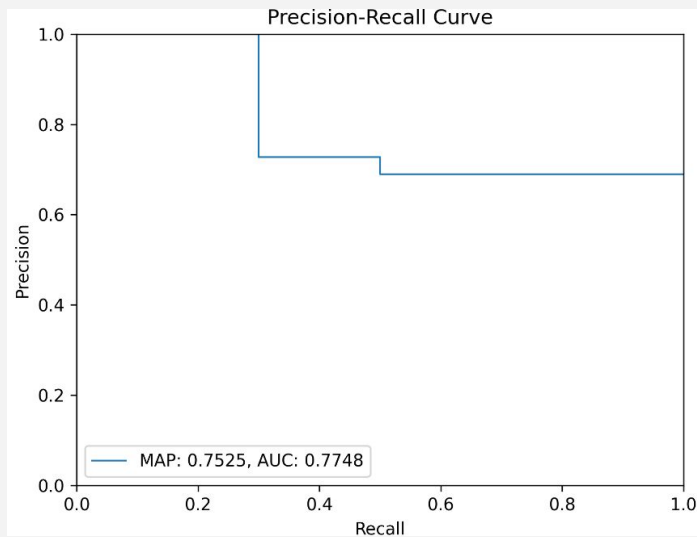
Query 1 - Improved Schema
