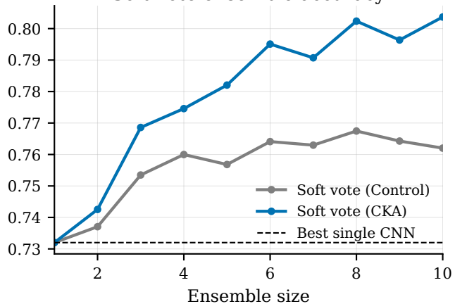
Soft-vote ensemble accuracy
