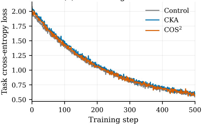
(a) Fine-tuning task loss
