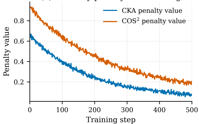
(b) Diversity penalty over training
