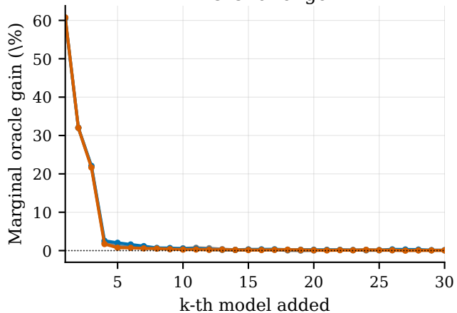
ARC-Challenge
