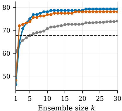
HumanEval
