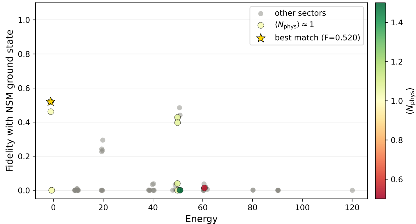
Gadget eigenstates — energy vs fidelity
