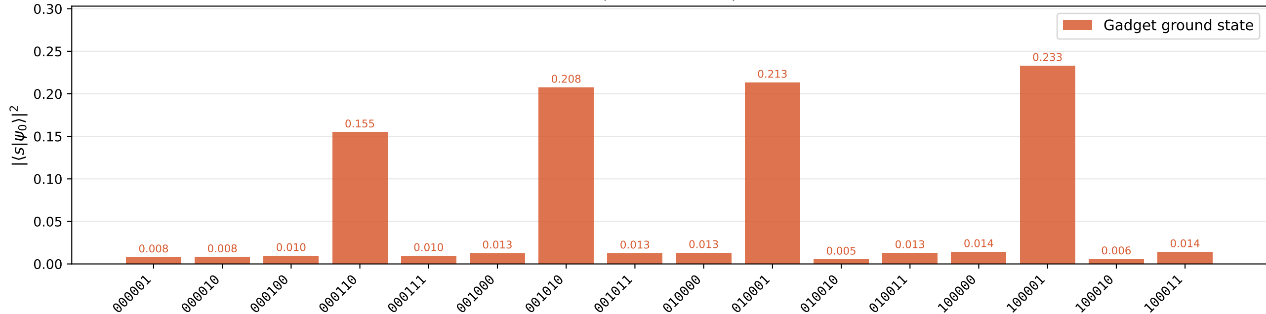
Top-16 components of total Hamiltonian ground state ( E = -4.769997 )
