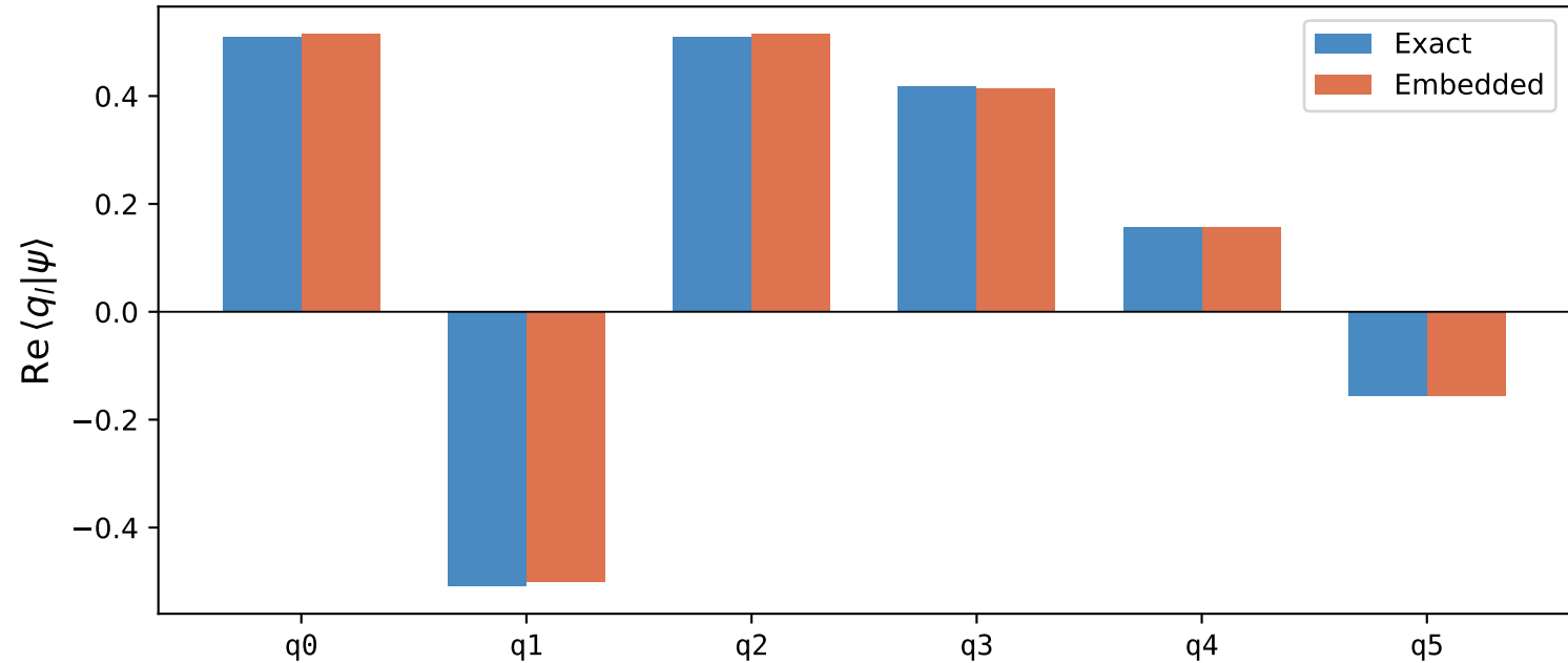
Real part of amplitudes — N=1 sector \gamma=200 , J_F=4000000.0 , Fidelity=0.99962
