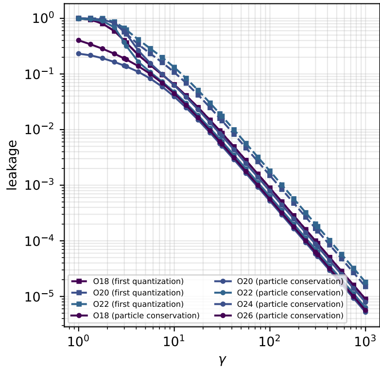
sd shell
