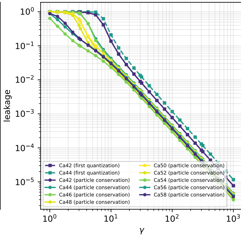
pf shell
